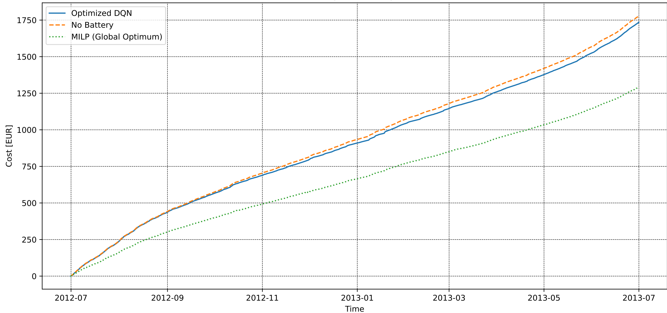
User 137 - Basic Training - Electricity Cost [DQN vs MILP]
